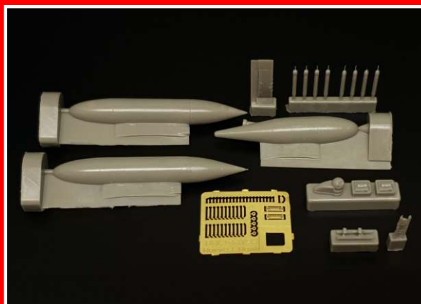
BRL144199 KC-130J Harvest Hawk conversion set for C-130 Hercules
