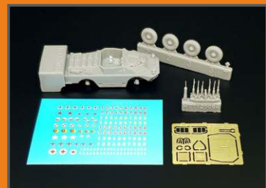
HTT120094 9P122 Maljutka - resin constr.kit of soviet AT vehicle
